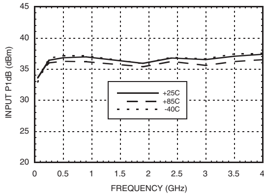
Input P1dB vs. Temperature, Vctl = 0/+3V
